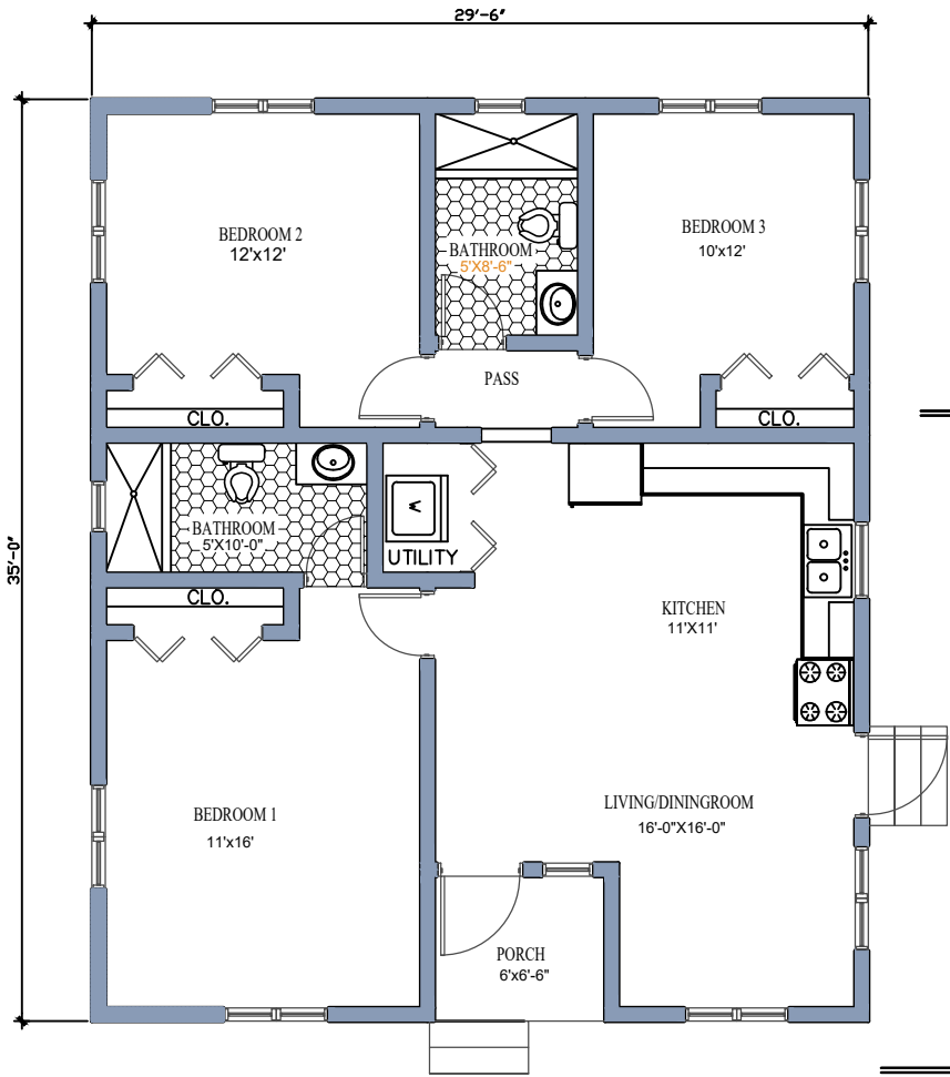
FLOOR PLAN 1,000 sq'
