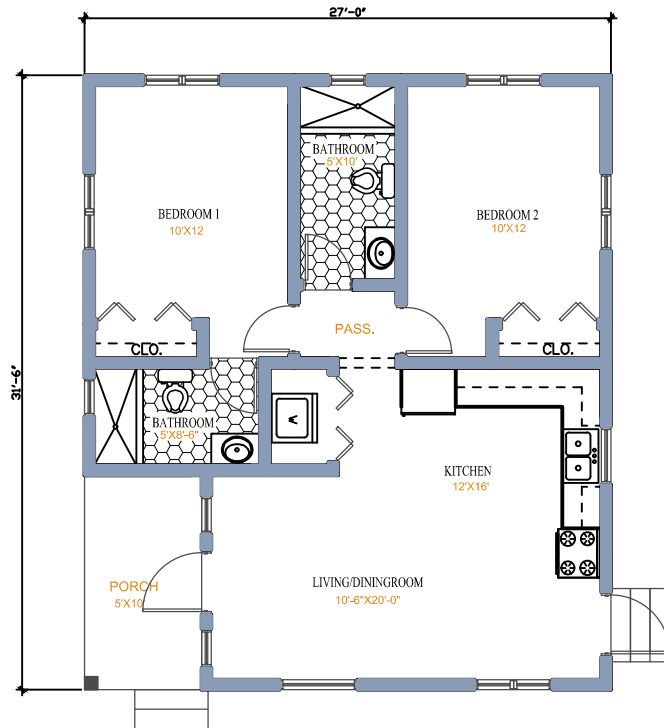
FLOOR PLAN 800 sq'
