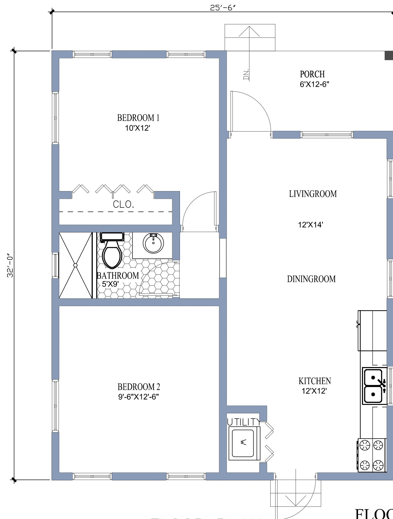
FLOOR PLAN 800 sq'
