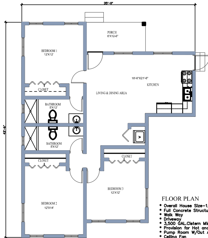
FLOOR PLAN SCALE: 3/16" = 1'-0"
