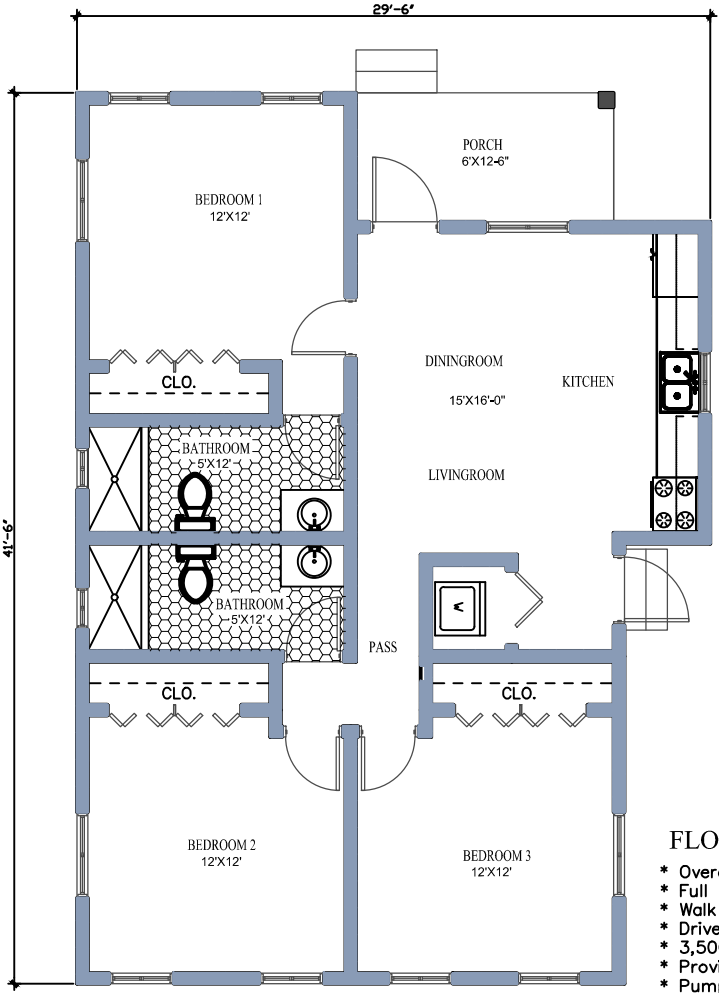
FLOOR PLAN 1,100 sq'
