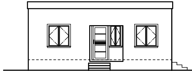
FRONT ELEVATION
