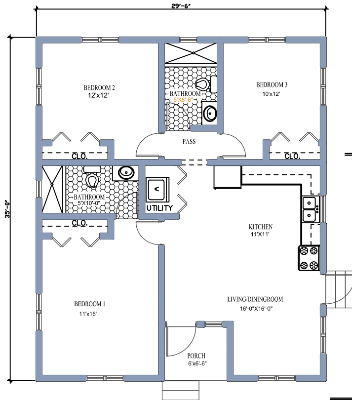
FLOOR PLAN 1,000 sq'
