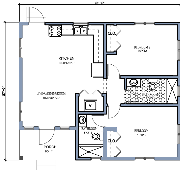
FLOOR PLAN 800 sq'
