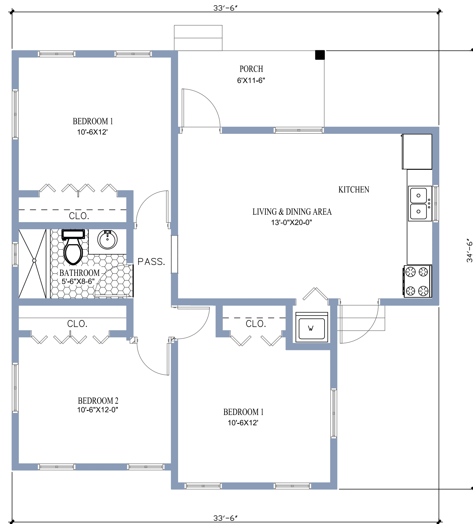
FLOOR PLAN 900 sq'
